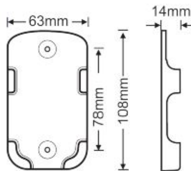
Remote holder
